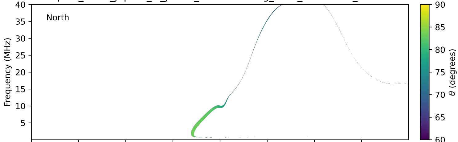
expres_earth_jupiter_io_jrm33_lossc-wid1deg_3kev_20260222_v11.cdf
