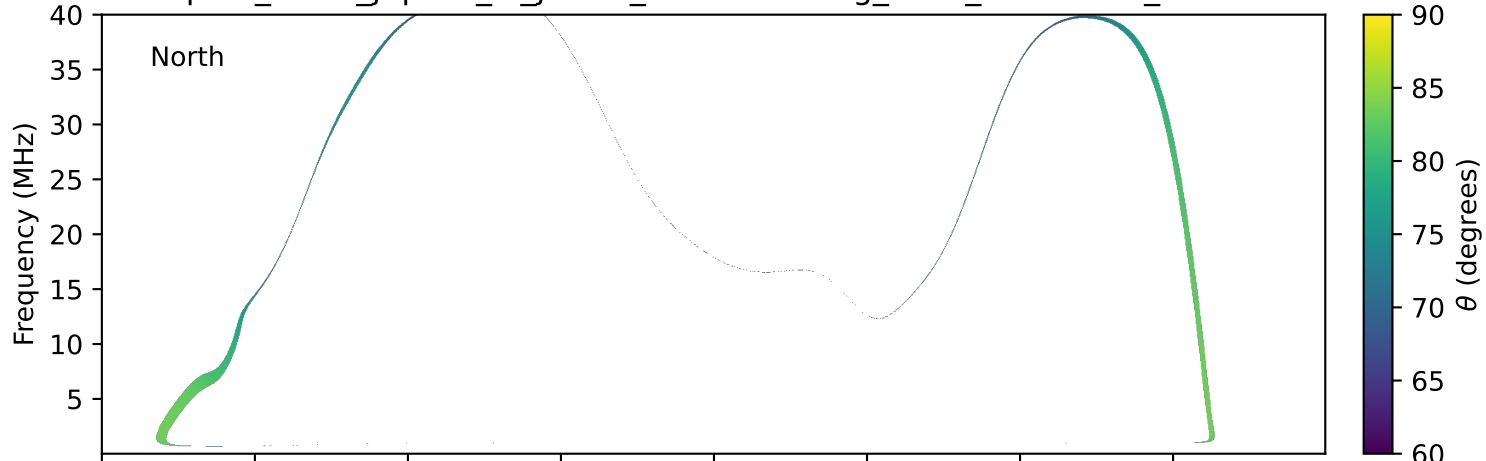
expres_earth_jupiter_io_jrm33_lossc-wid1deg_3kev_20260210_v11.cdf
