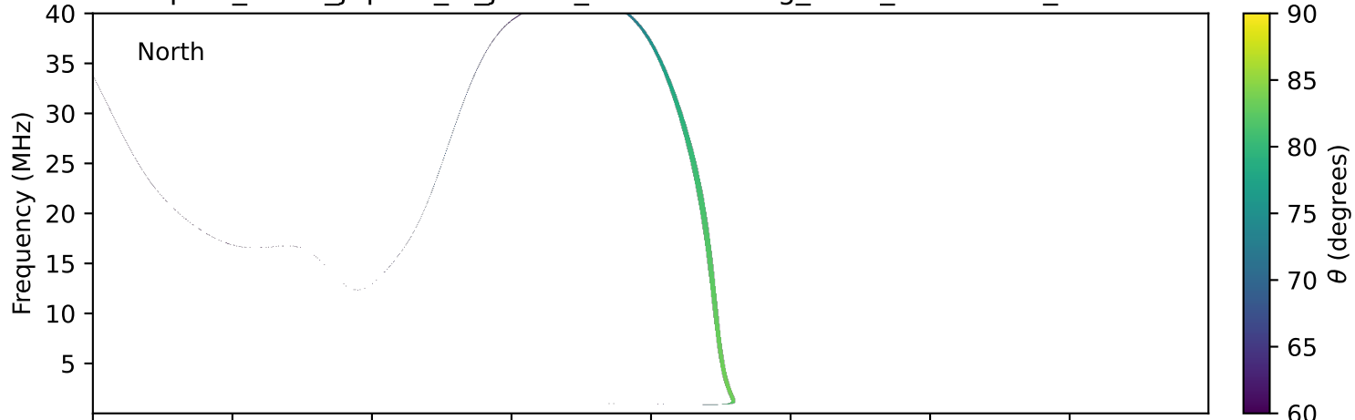
expres_earth_jupiter_io_jrm33_lossc-wid1deg_3kev_20260205_v11.cdf
