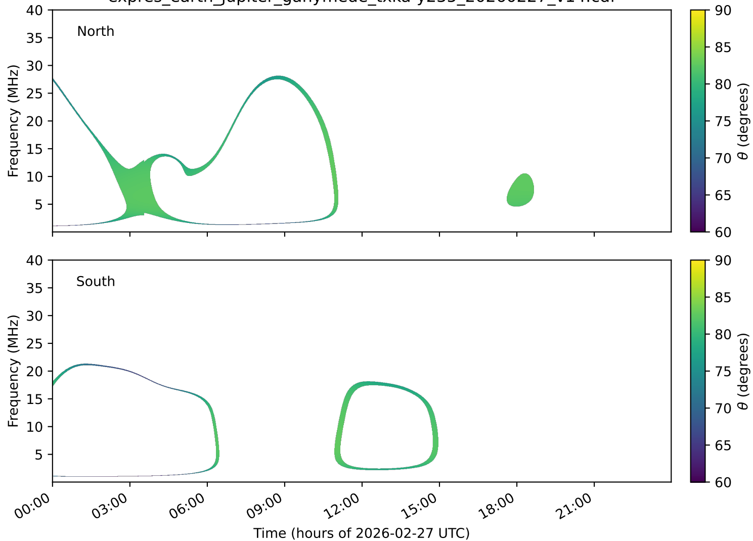
expres_earth_jupiter_ganymede_txka-y235_20260227_v14.cdf
