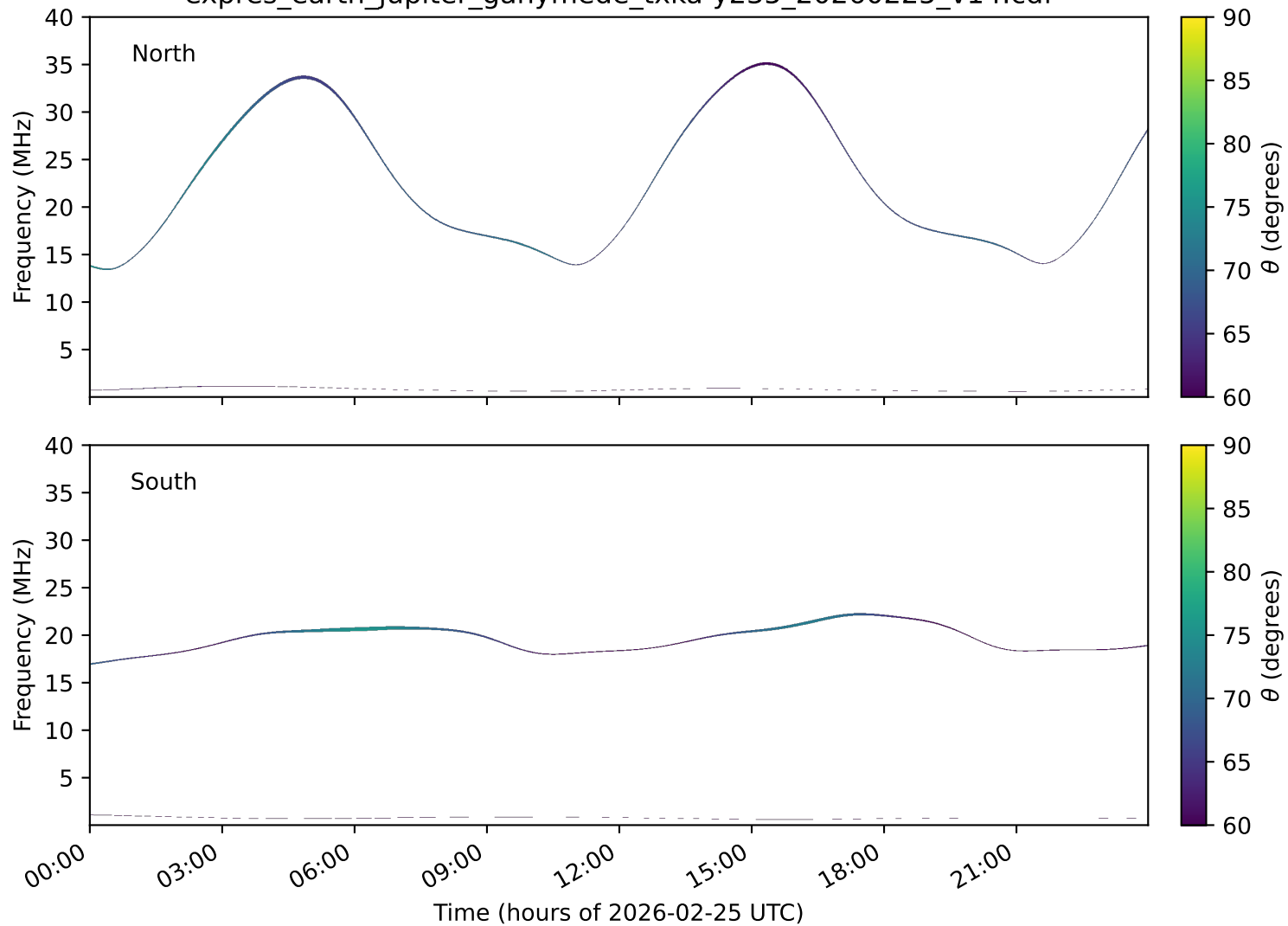
expres_earth_jupiter_ganymede_txka-y235_20260225_v14.cdf
