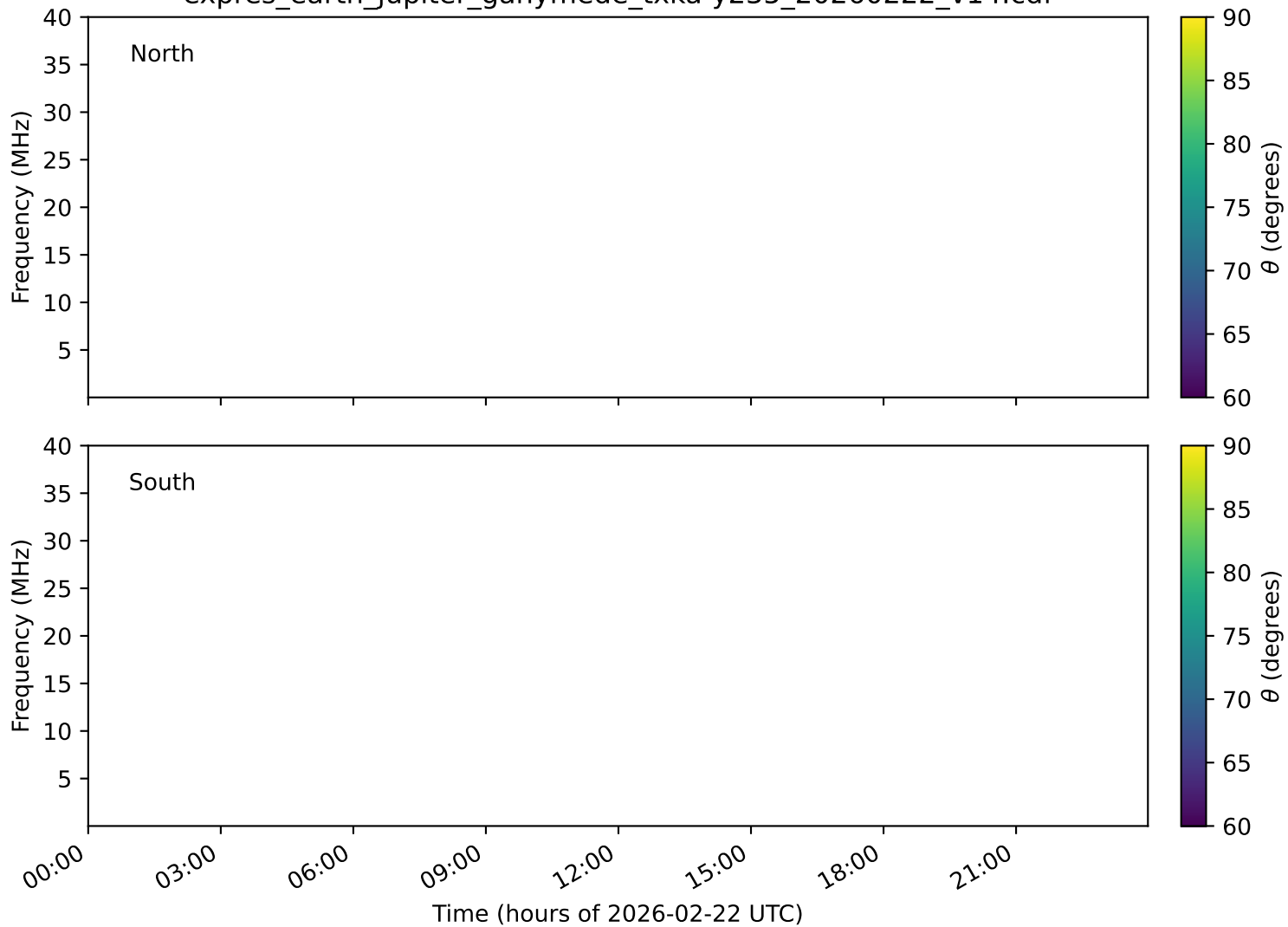
expres_earth_jupiter_ganymede_txka-y235_20260222_v14.cdf
