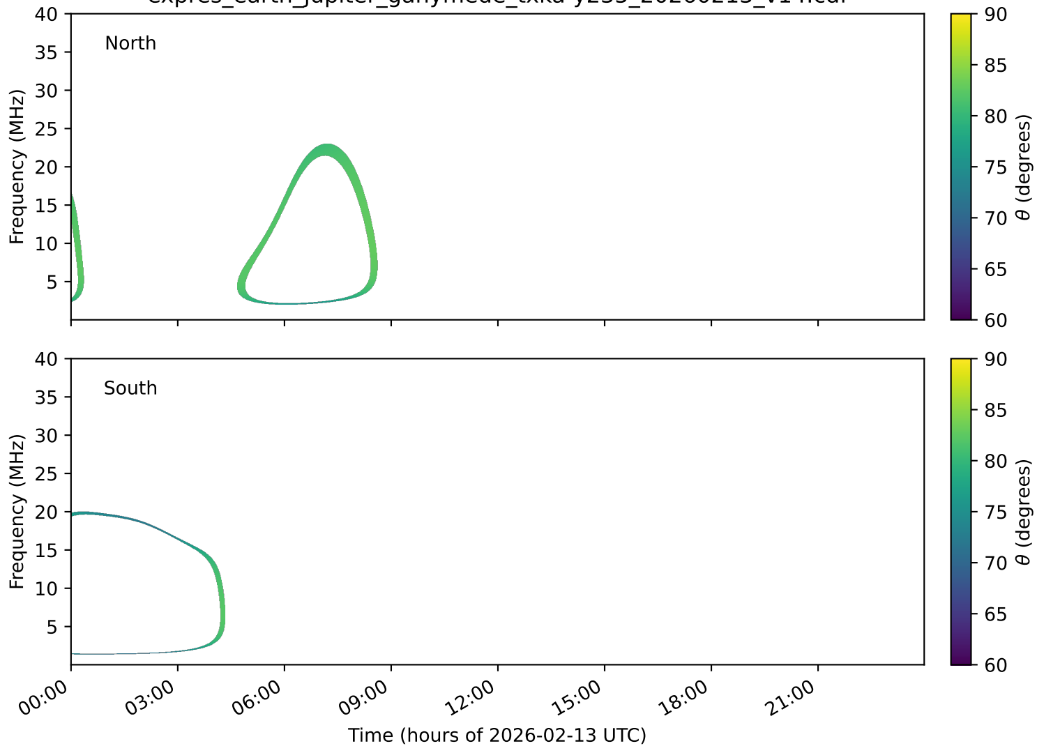
expres_earth_jupiter_ganymede_txka-y235_20260213_v14.cdf
