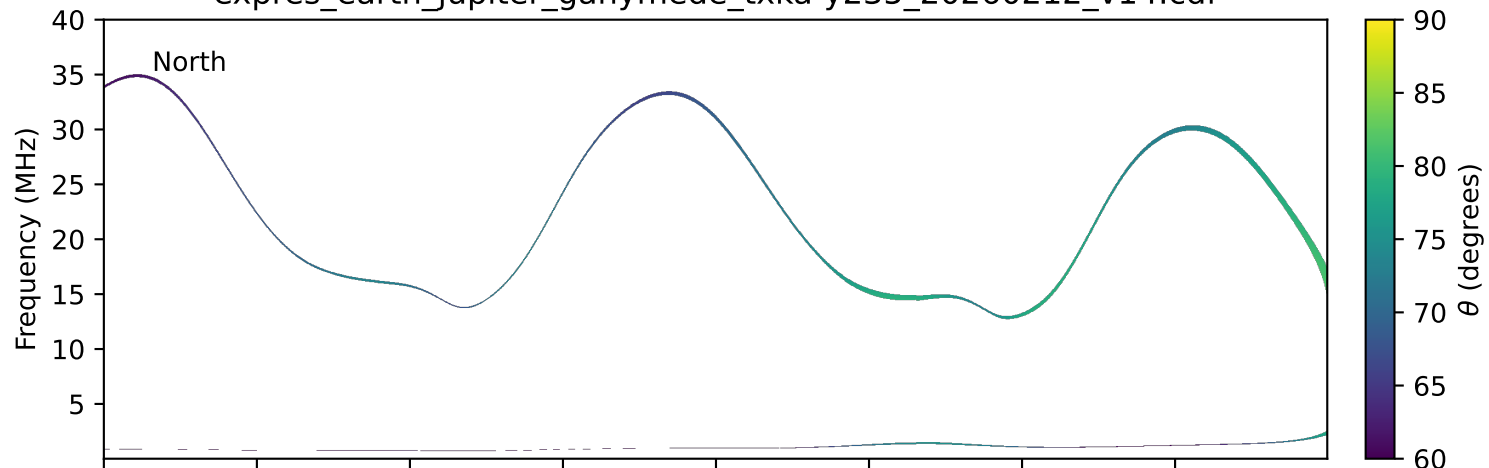
expres_earth_jupiter_ganymede_txka-y235_20260212_v14.cdf
