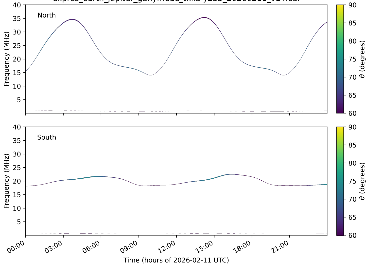
expres_earth_jupiter_ganymede_txka-y235_20260211_v14.cdf
