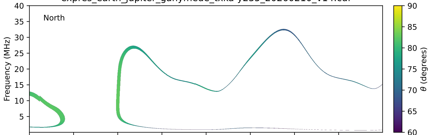
expres_earth_jupiter_ganymede_txka-y235_20260210_v14.cdf
