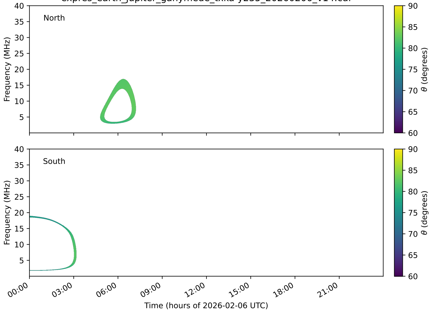
expres_earth_jupiter_ganymede_txka-y235_20260206_v14.cdf
