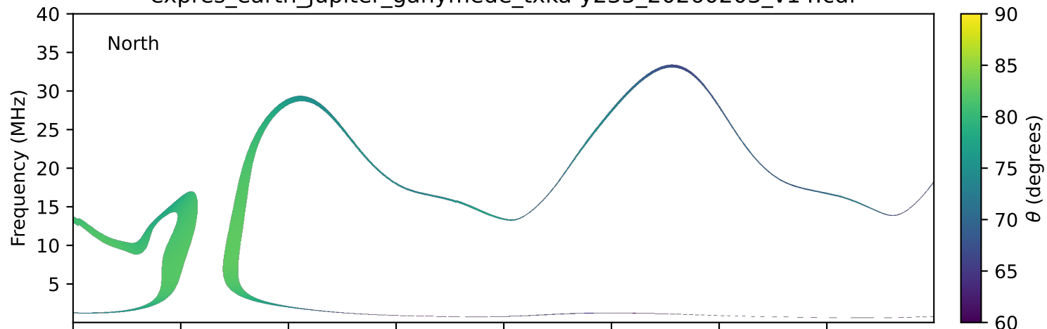
expres_earth_jupiter_ganymede_txka-y235_20260203_v14.cdf
