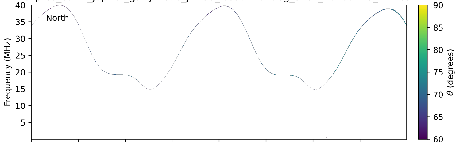
expres_earth_jupiter_ganymede_jrm33_lossc-wid1deg_3kev_20260226_v11.cdf
