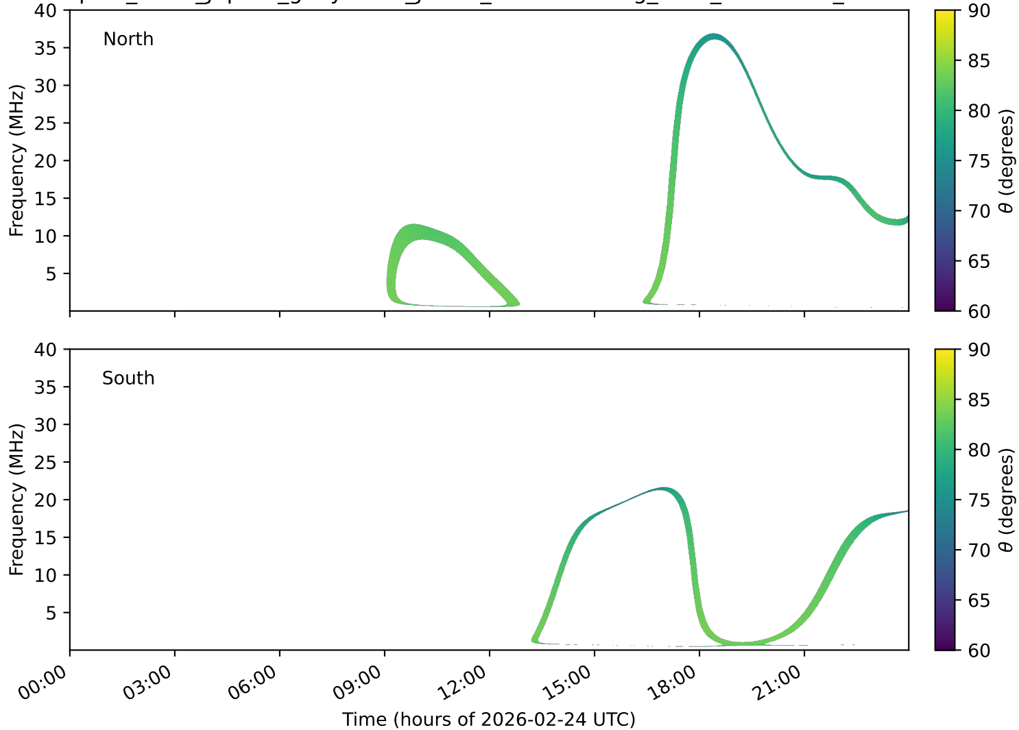
expres_earth_jupiter_ganymede_jrm33_lossc-wid1deg_3kev_20260224_v11.cdf
