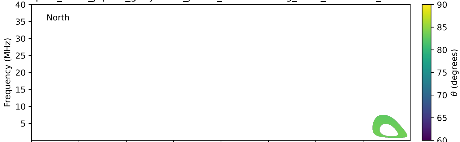
expres_earth_jupiter_ganymede_jrm33_lossc-wid1deg_3kev_20260202_v11.cdf
