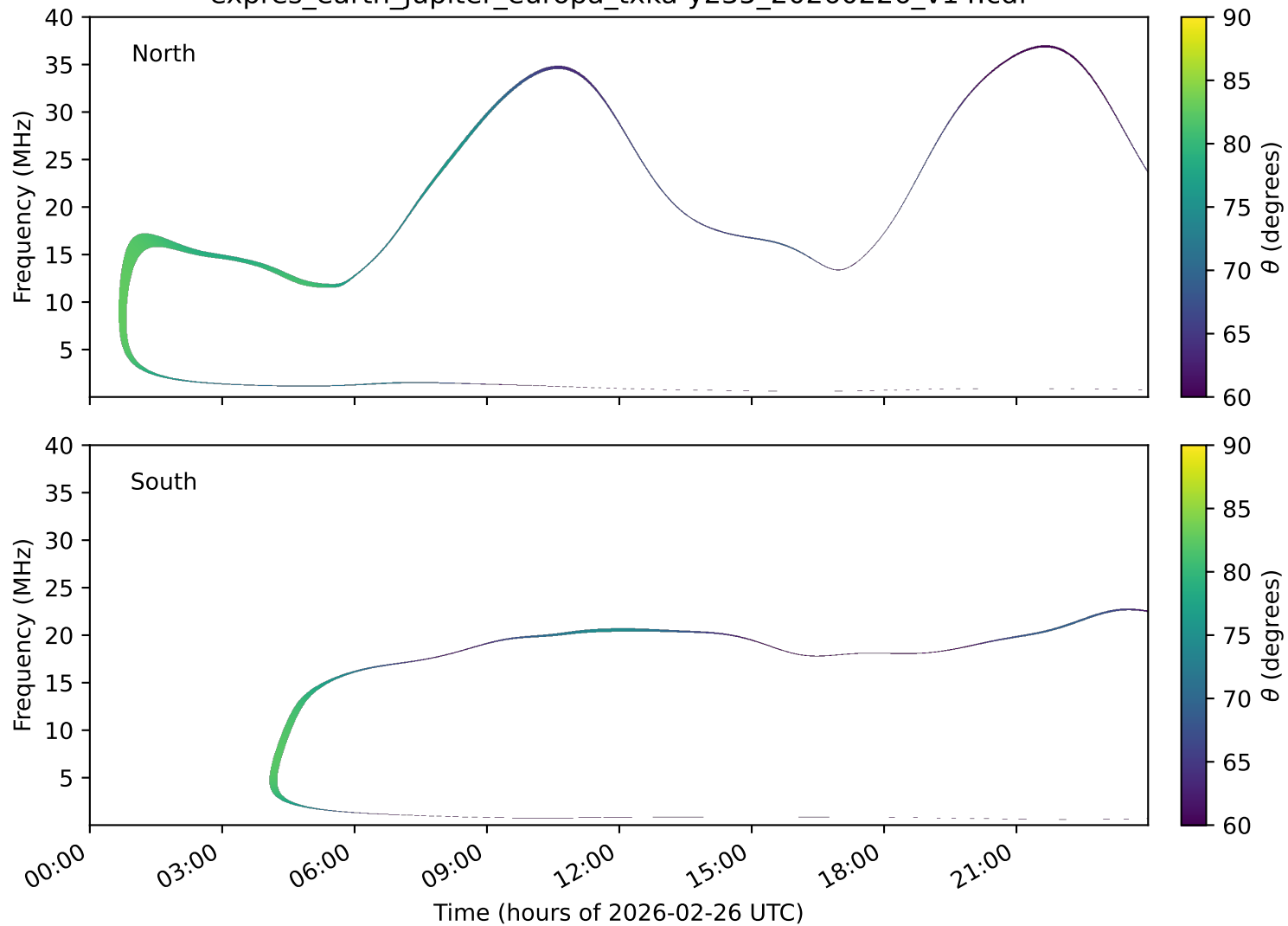
expres_earth_jupiter_europa_txka-y235_20260226_v14.cdf
