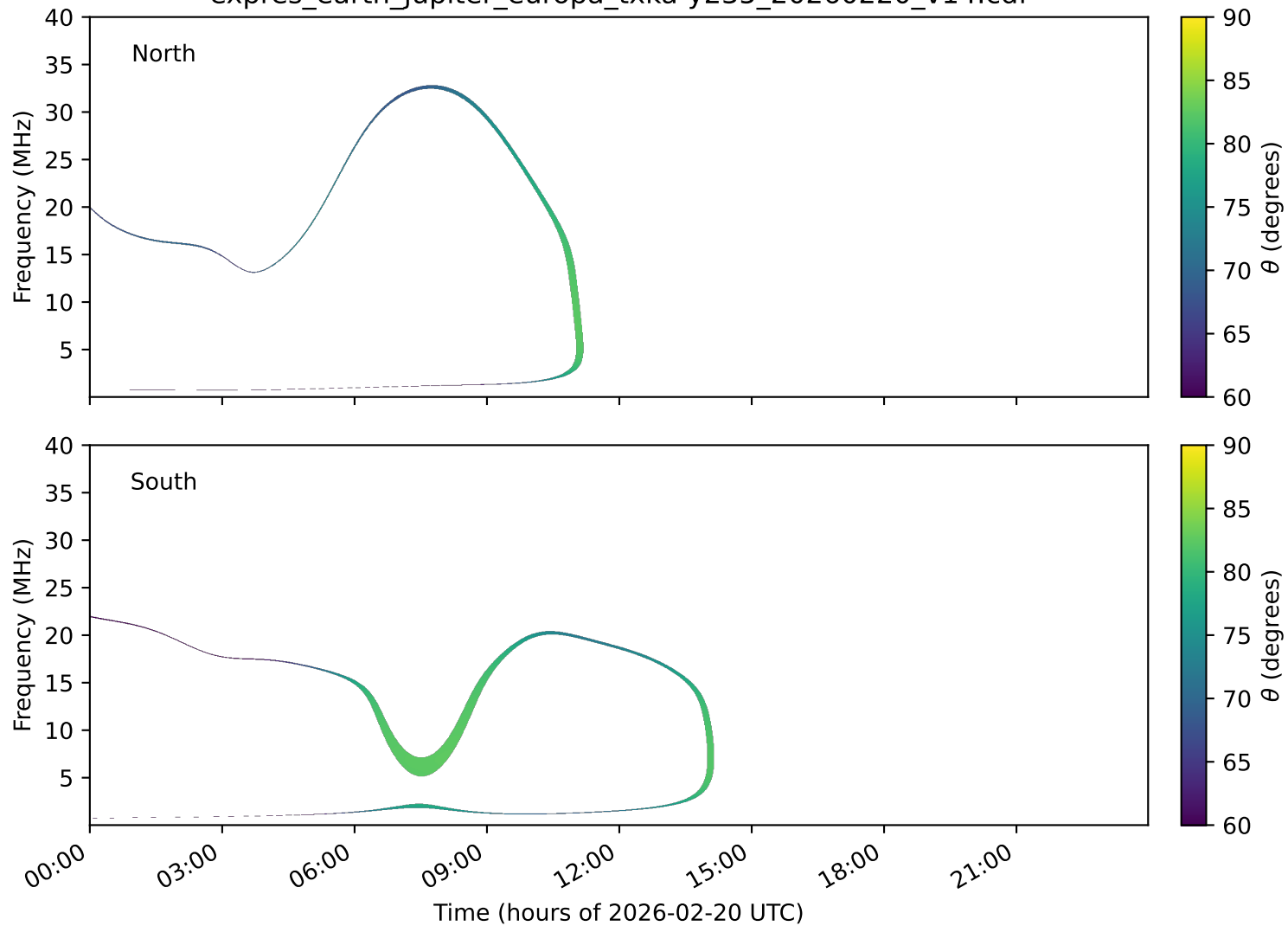
expres_earth_jupiter_europa_txka-y235_20260220_v14.cdf
