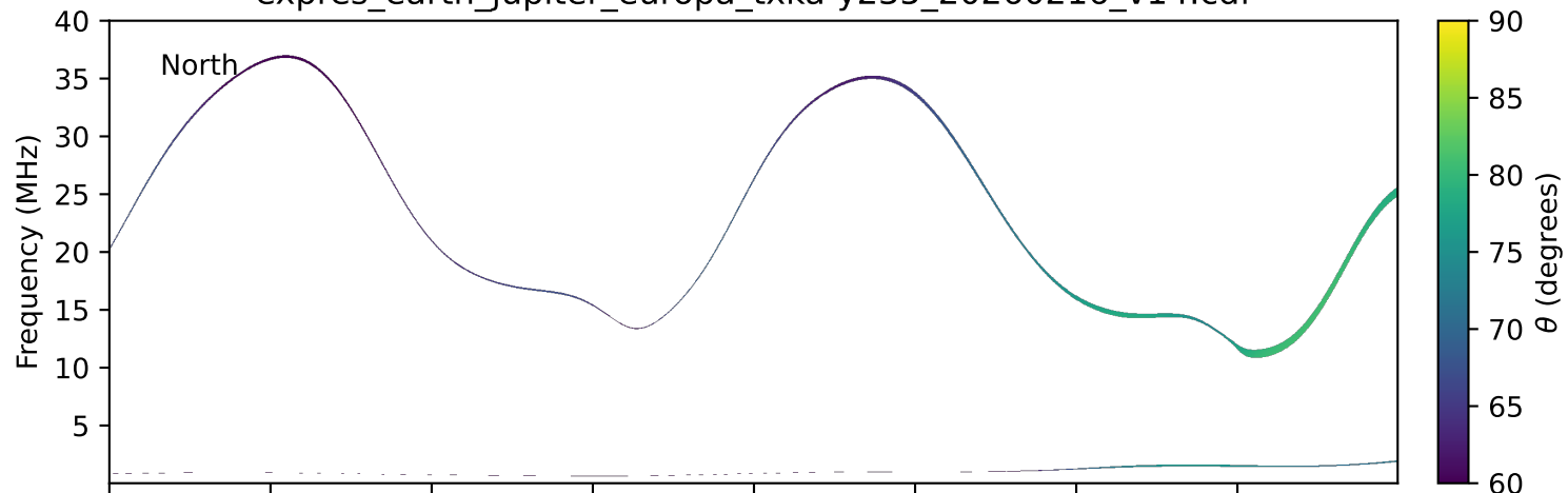
expres_earth_jupiter_europa_txka-y235_20260216_v14.cdf
