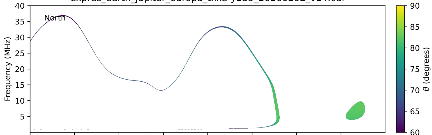
expres_earth_jupiter_europa_txka-y235_20260202_v14.cdf
