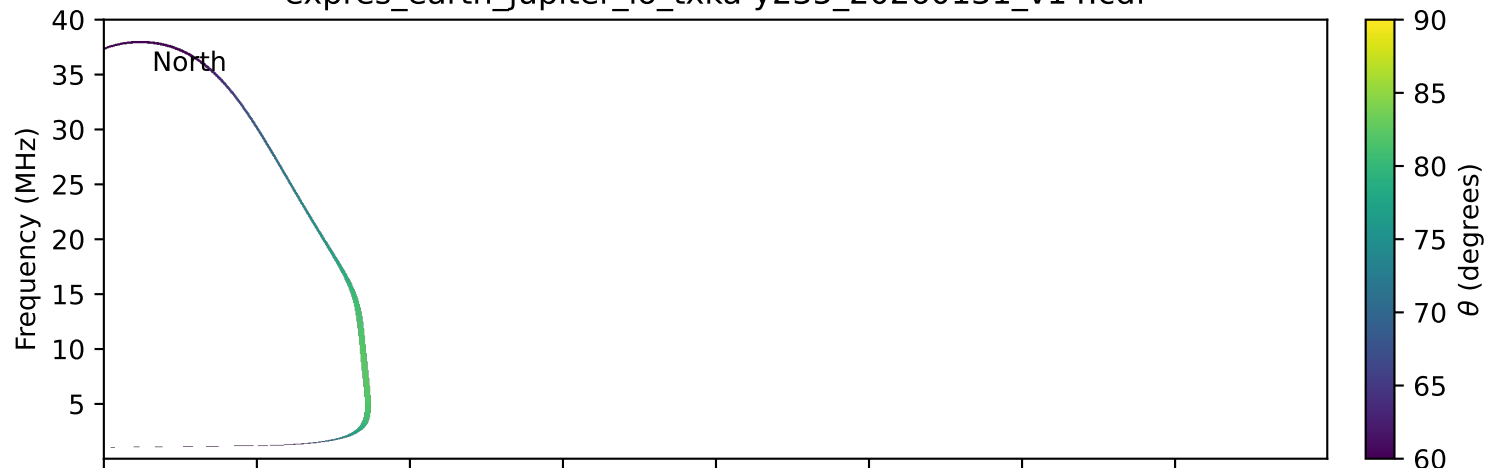
expres_earth_jupiter_io_txka-y235_20260131_v14.cdf
