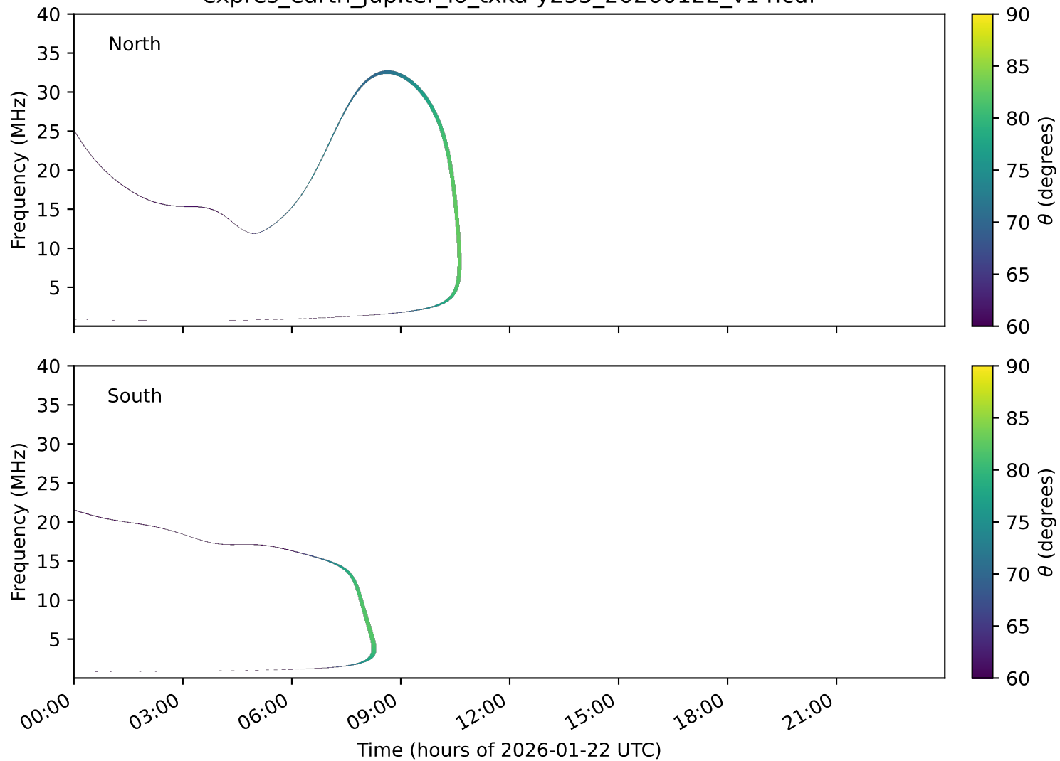
expres_earth_jupiter_io_txka-y235_20260122_v14.cdf
