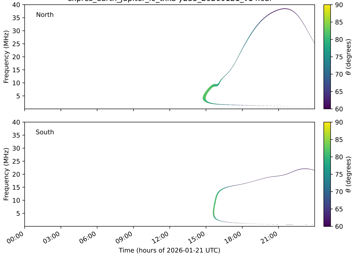
expres_earth_jupiter_io_txka-y235_20260121_v14.cdf
