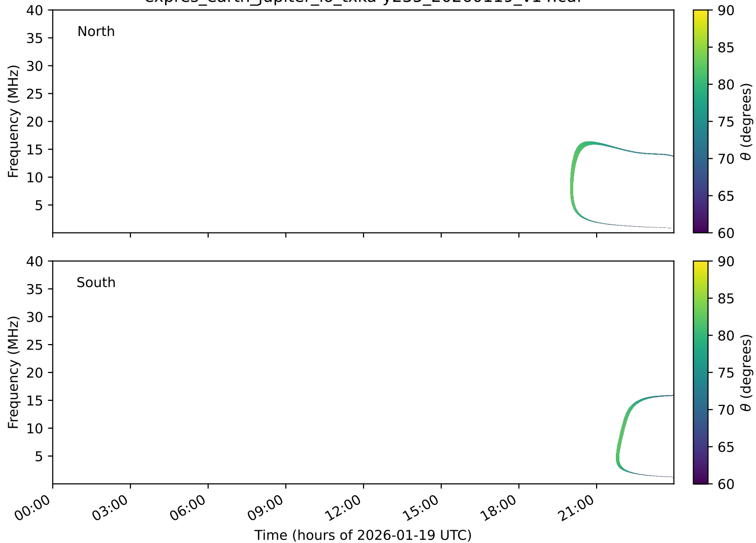
expres_earth_jupiter_io_txka-y235_20260119_v14.cdf
