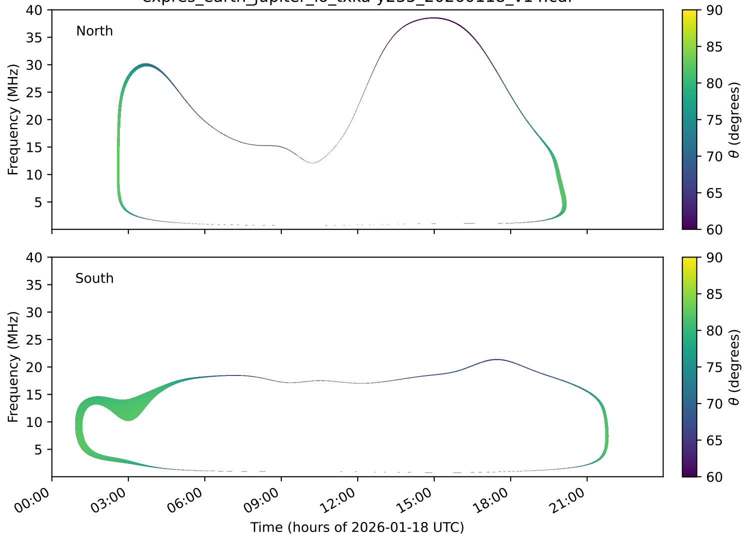
expres_earth_jupiter_io_txka-y235_20260118_v14.cdf
