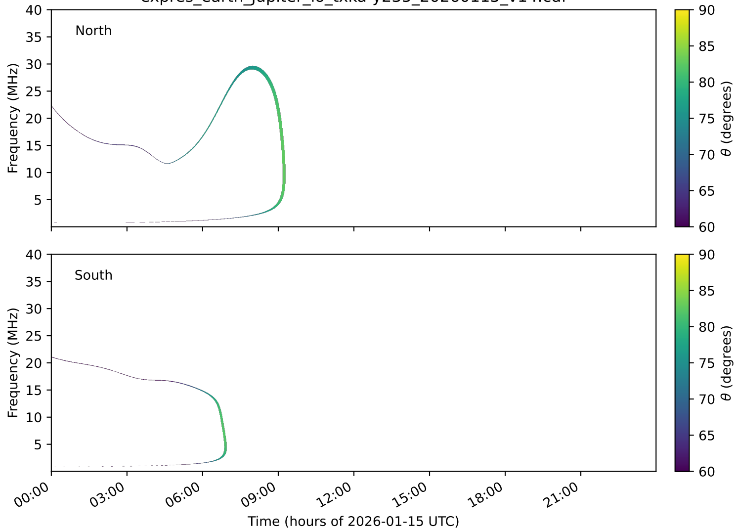
expres_earth_jupiter_io_txka-y235_20260115_v14.cdf
