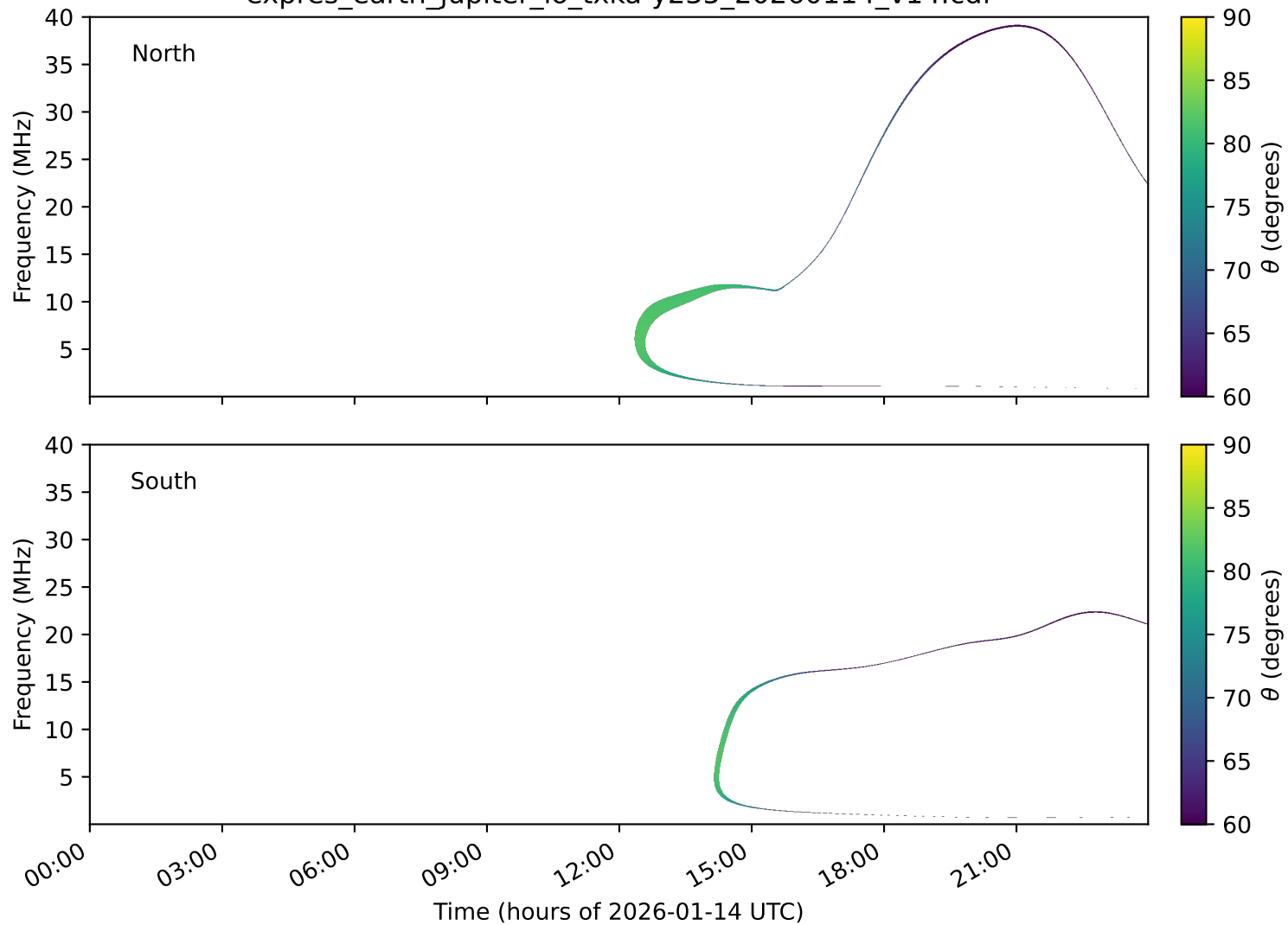
expres_earth_jupiter_io_txka-y235_20260114_v14.cdf
