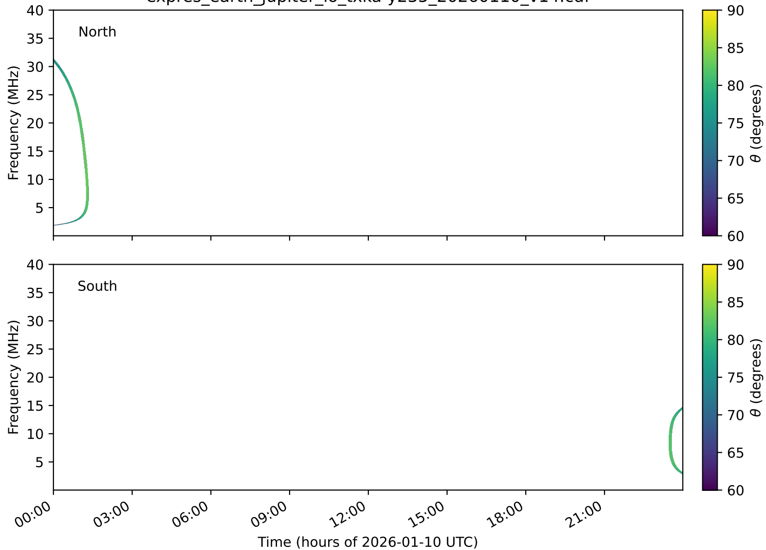
expres_earth_jupiter_io_txka-y235_20260110_v14.cdf
