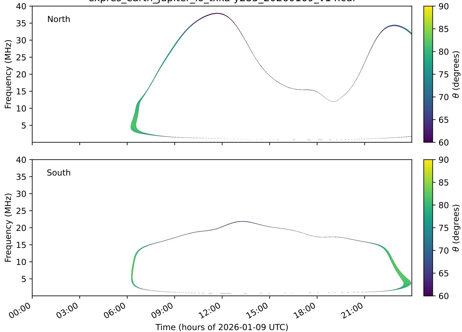
expres_earth_jupiter_io_txka-y235_20260109_v14.cdf
