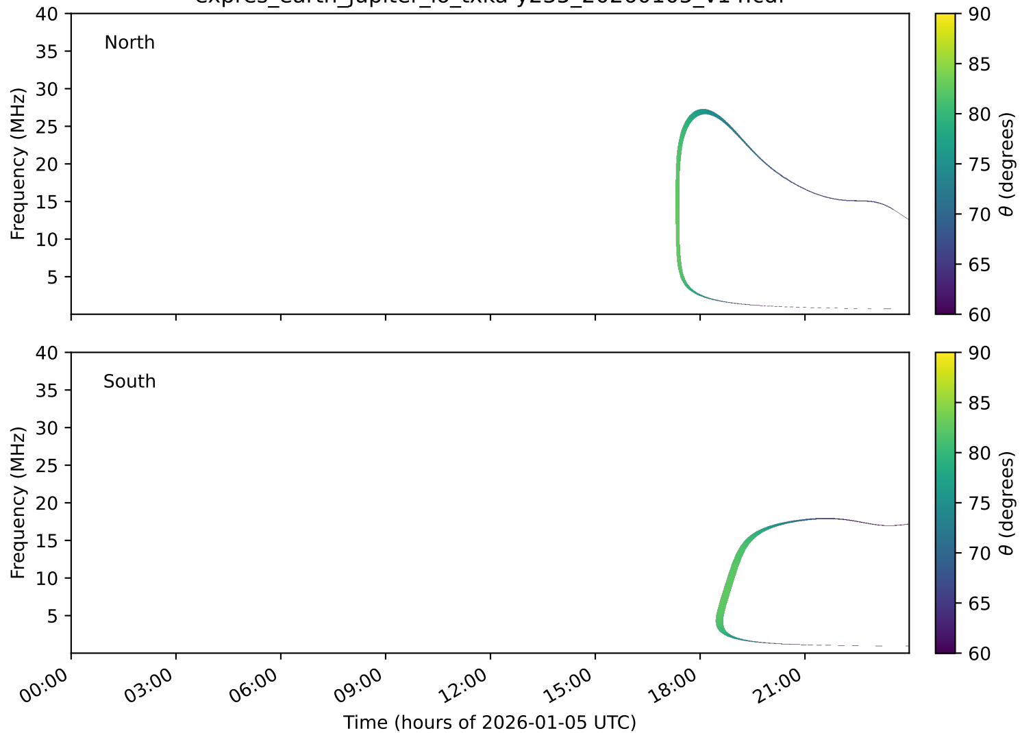
expres_earth_jupiter_io_txka-y235_20260105_v14.cdf
