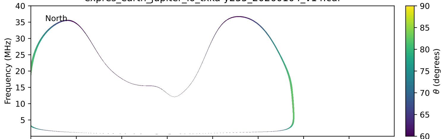
expres_earth_jupiter_io_txka-y235_20260104_v14.cdf
