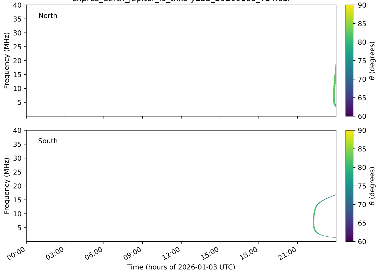
expres_earth_jupiter_io_txka-y235_20260103_v14.cdf
