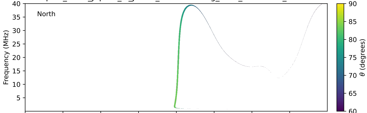
expres_earth_jupiter_io_jrm33_lossc-wid1deg_3kev_20260130_v11.cdf
