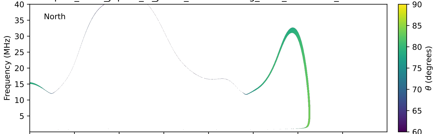
expres_earth_jupiter_io_jrm33_lossc-wid1deg_3kev_20260127_v11.cdf
