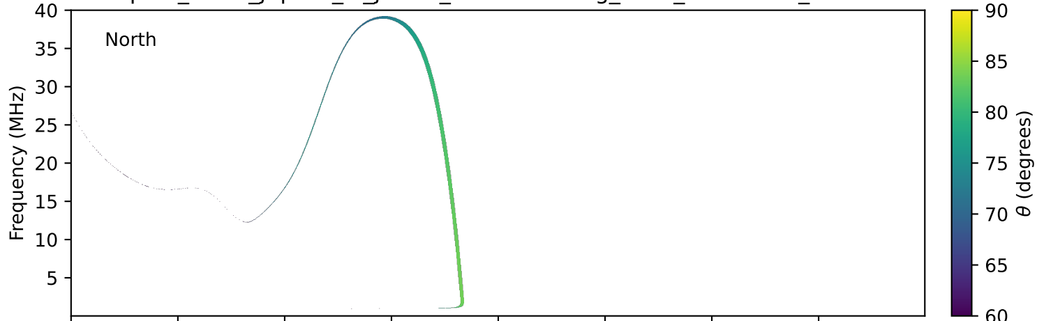
expres_earth_jupiter_io_jrm33_lossc-wid1deg_3kev_20260122_v11.cdf
