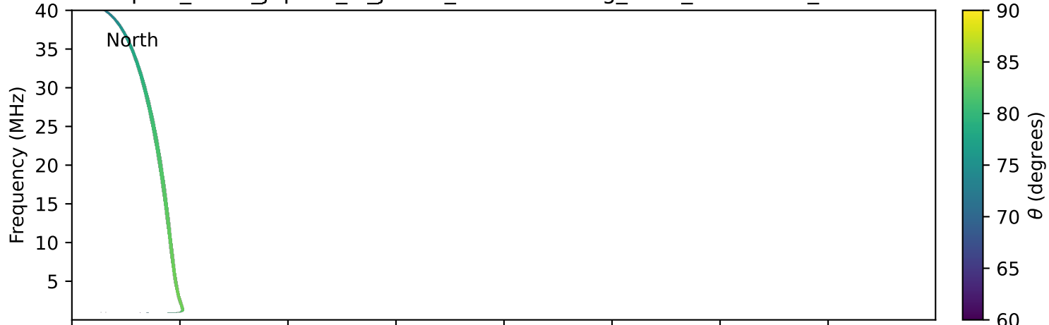
expres_earth_jupiter_io_jrm33_lossc-wid1deg_3kev_20260117_v11.cdf
