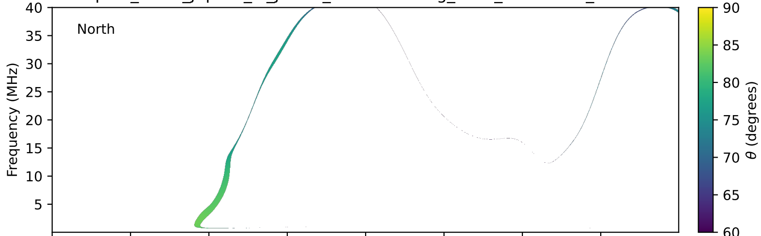
expres_earth_jupiter_io_jrm33_lossc-wid1deg_3kev_20260109_v11.cdf
