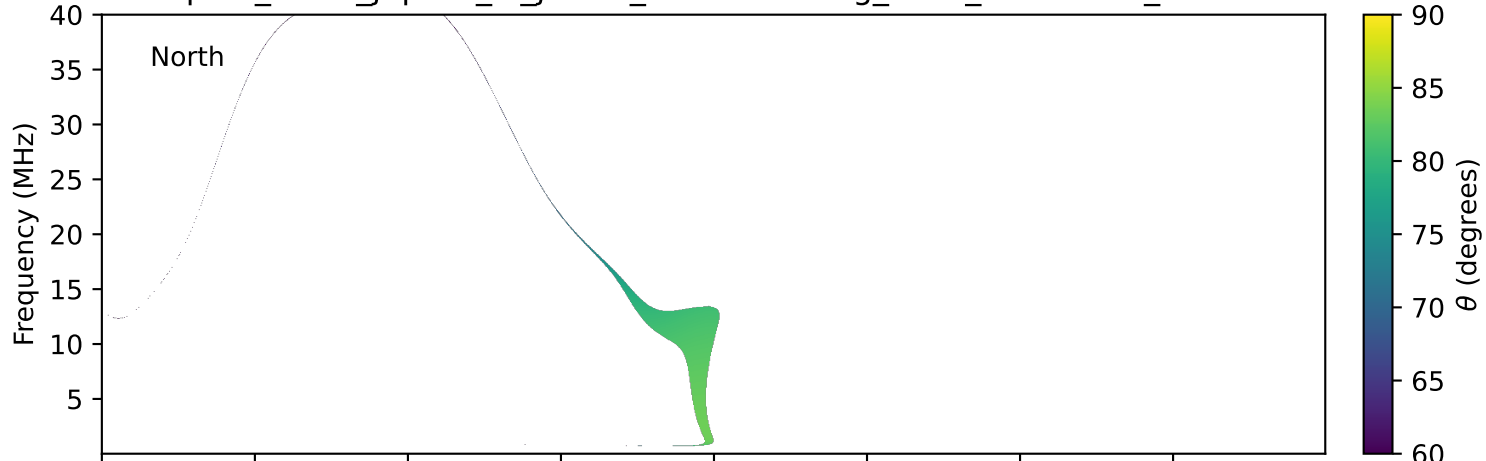
expres_earth_jupiter_io_jrm33_lossc-wid1deg_3kev_20260106_v11.cdf
