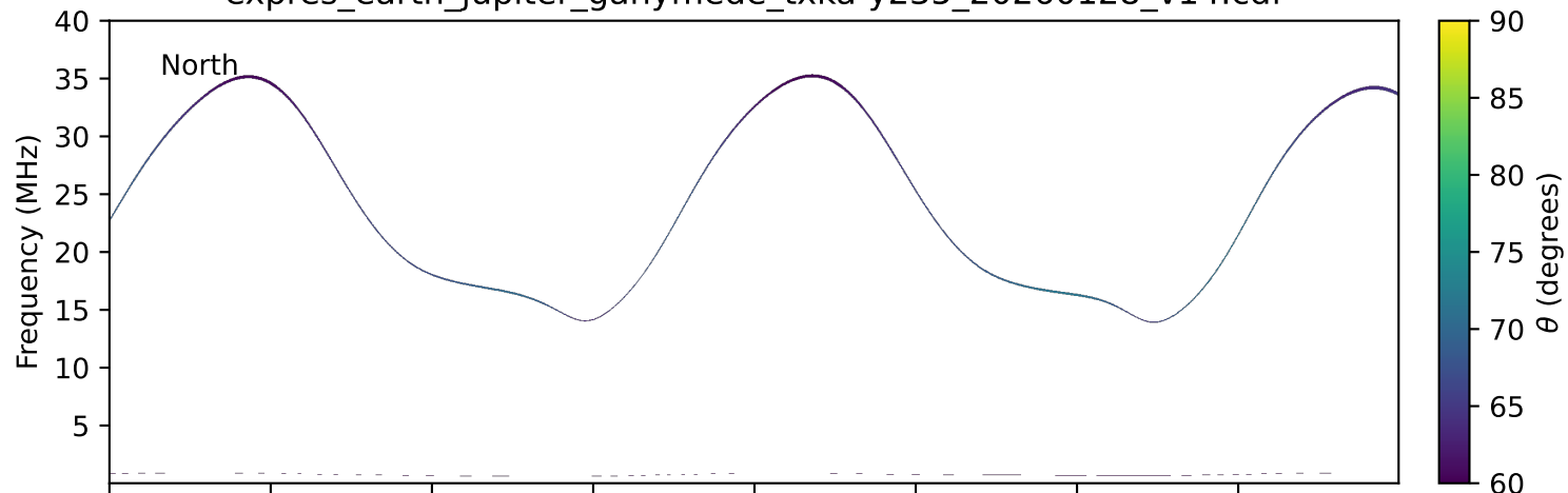
expres_earth_jupiter_ganymede_txka-y235_20260128_v14.cdf
