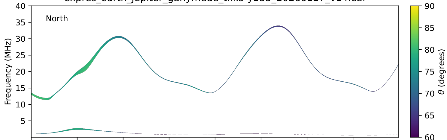
expres_earth_jupiter_ganymede_txka-y235_20260127_v14.cdf
