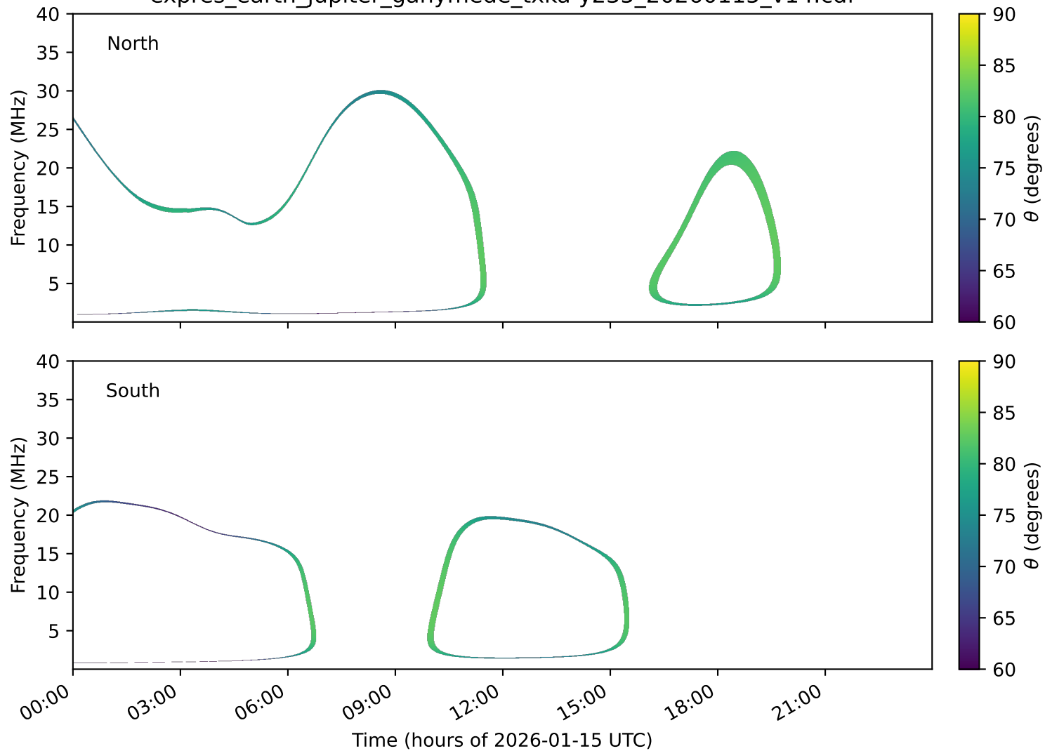
expres_earth_jupiter_ganymede_txka-y235_20260115_v14.cdf
