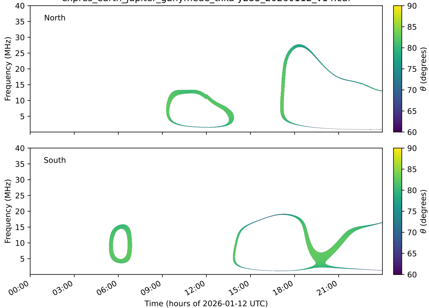
expres_earth_jupiter_ganymede_txka-y235_20260112_v14.cdf
