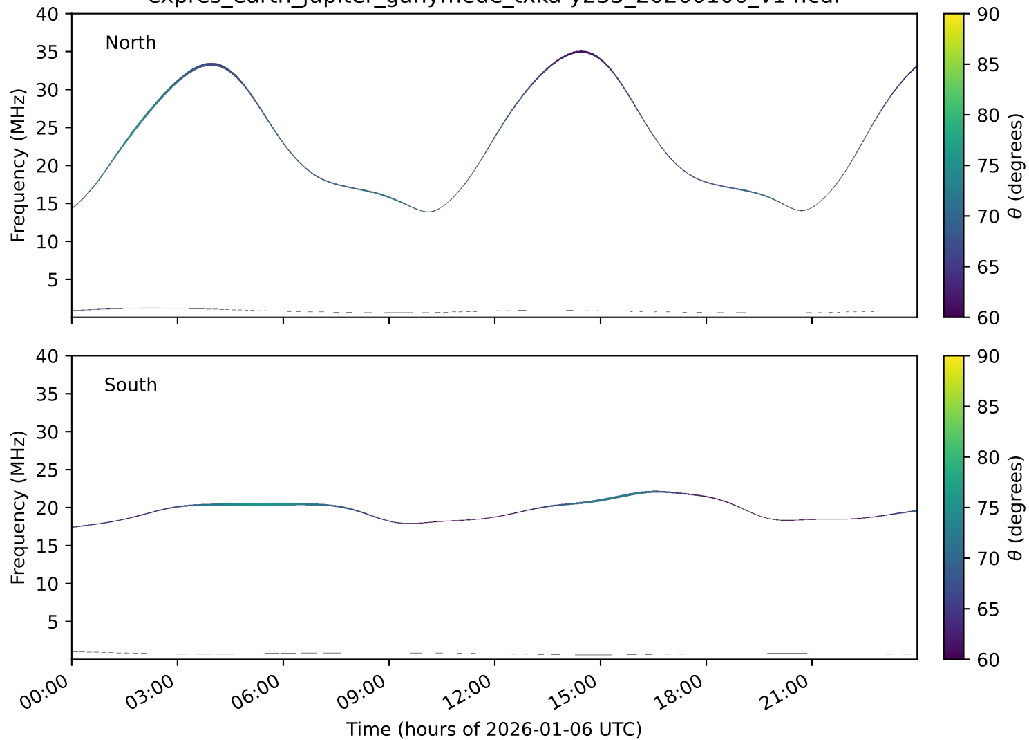
expres_earth_jupiter_ganymede_txka-y235_20260106_v14.cdf
