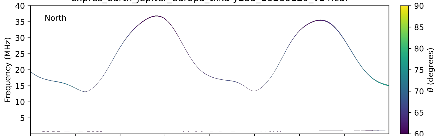
expres_earth_jupiter_europa_txka-y235_20260129_v14.cdf
