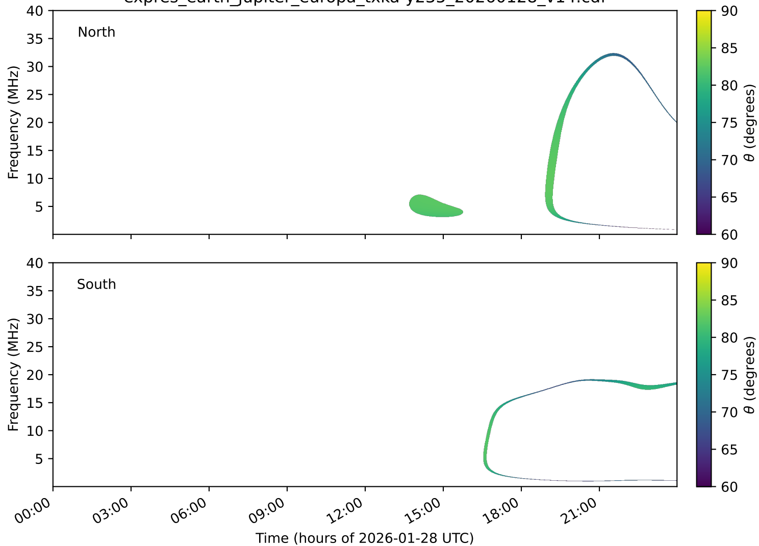
expres_earth_jupiter_europa_txka-y235_20260128_v14.cdf
