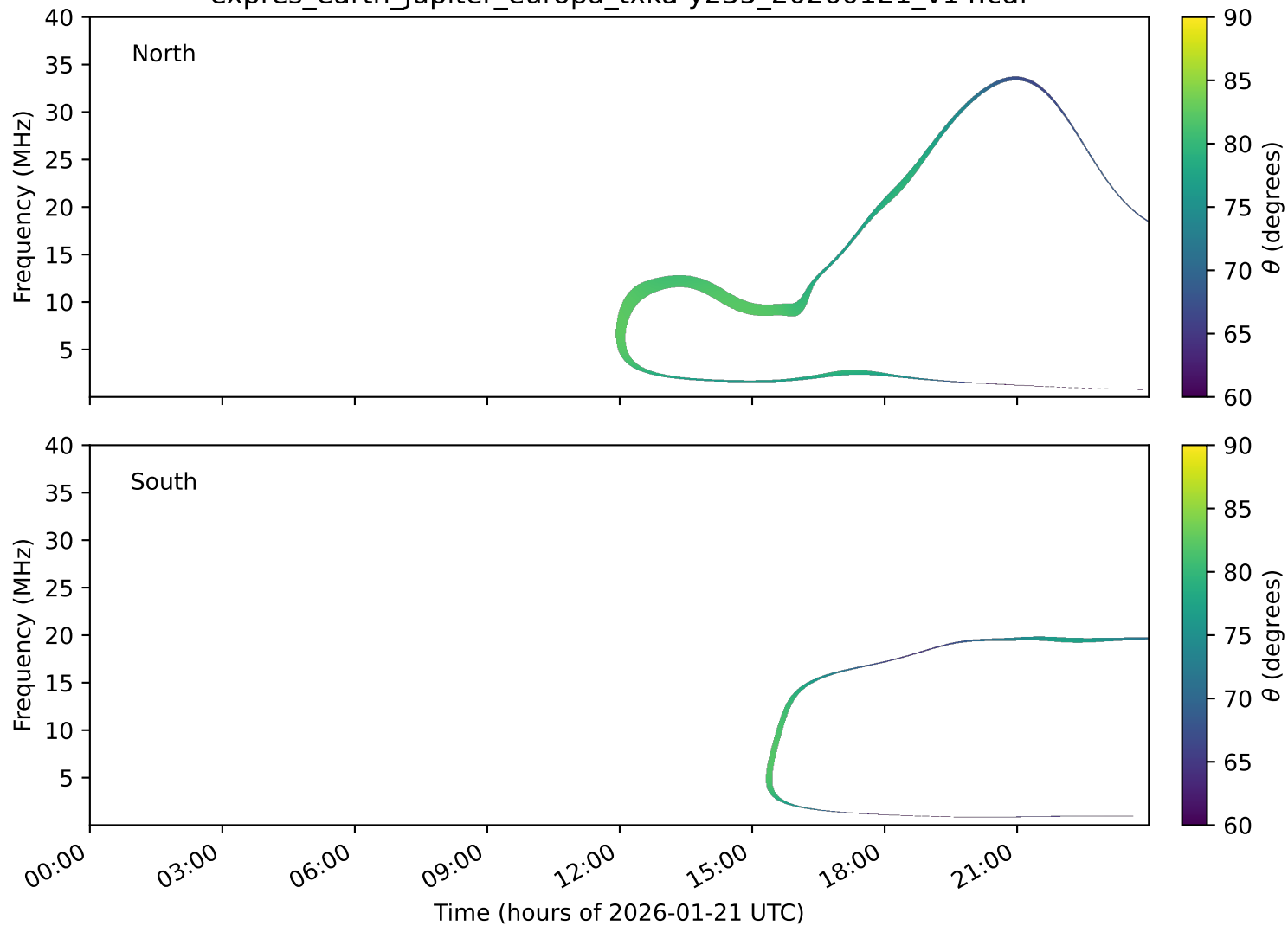
expres_earth_jupiter_europa_txka-y235_20260121_v14.cdf
