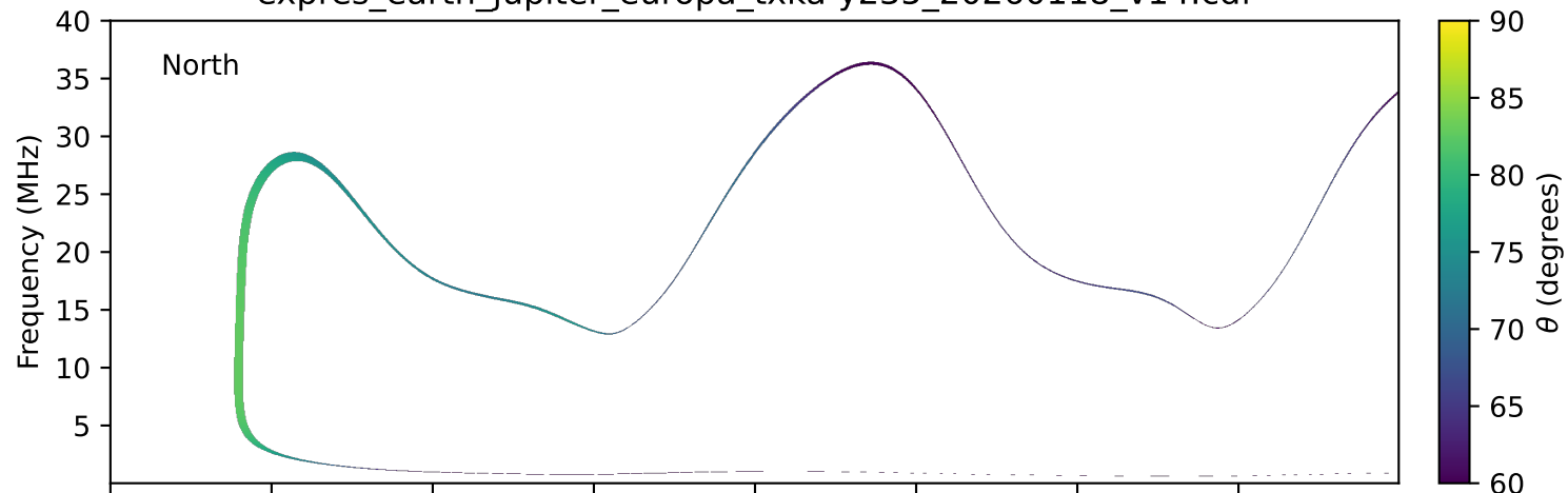
expres_earth_jupiter_europa_txka-y235_20260118_v14.cdf
