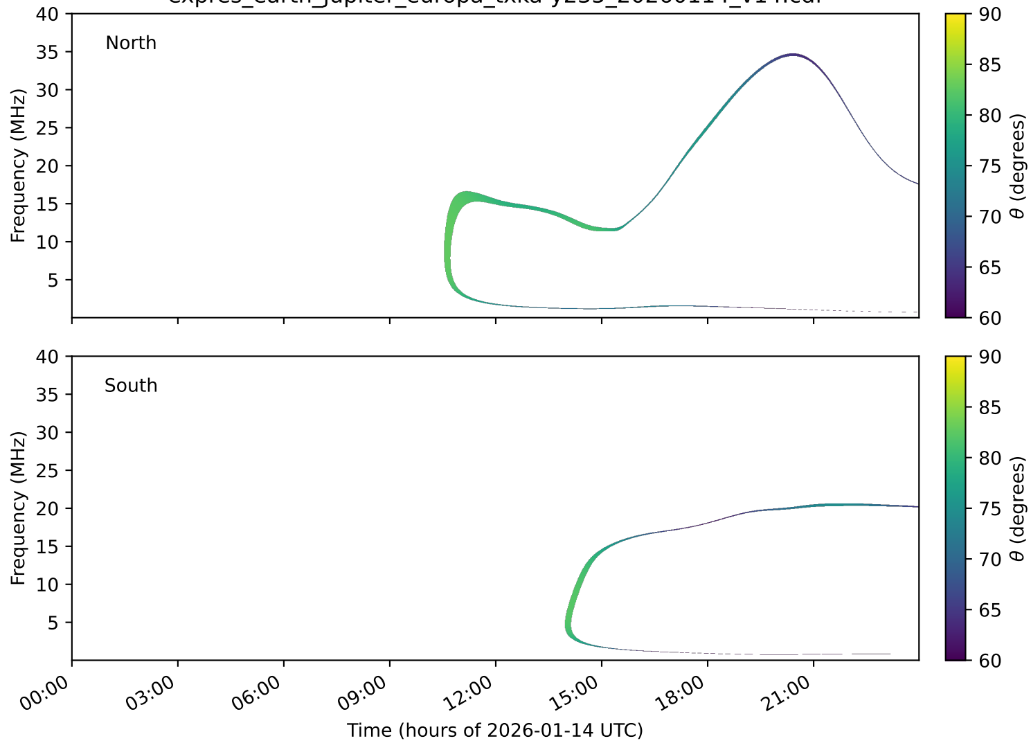
expres_earth_jupiter_europa_txka-y235_20260114_v14.cdf
