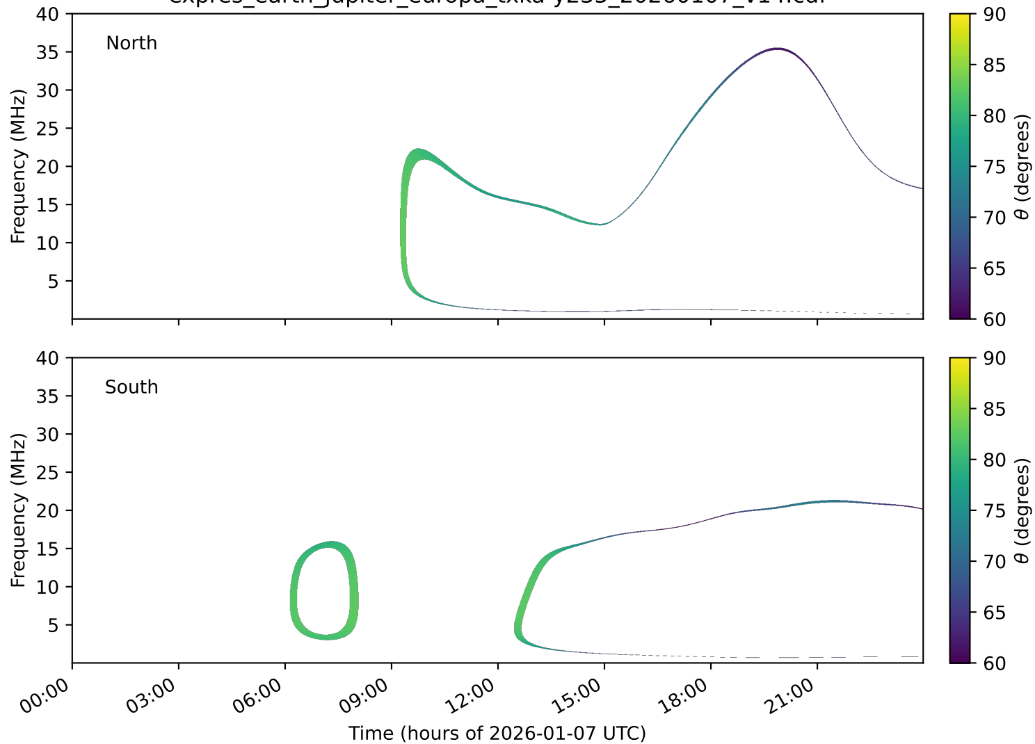
expres_earth_jupiter_europa_txka-y235_20260107_v14.cdf
