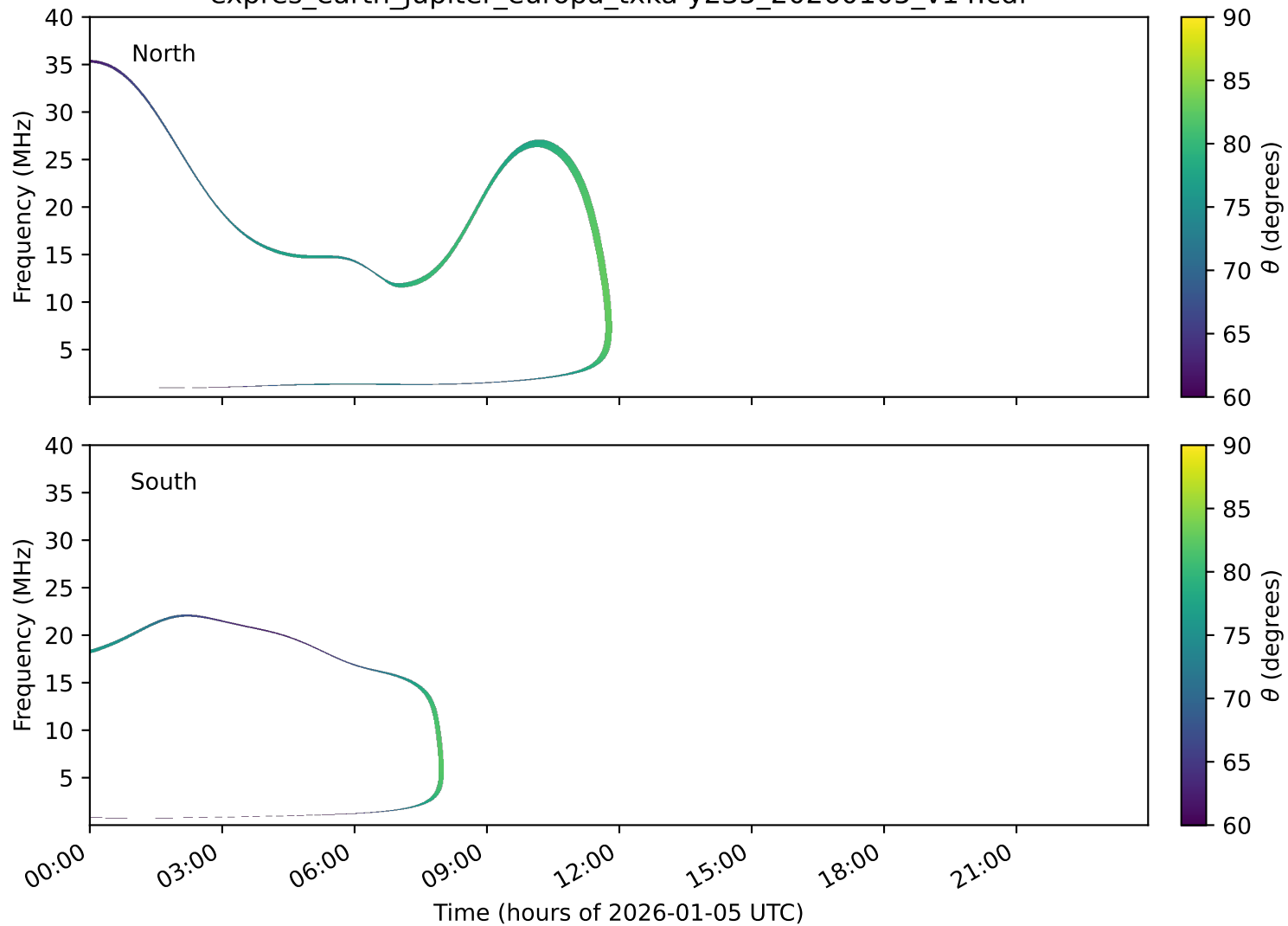
expres_earth_jupiter_europa_txka-y235_20260105_v14.cdf
