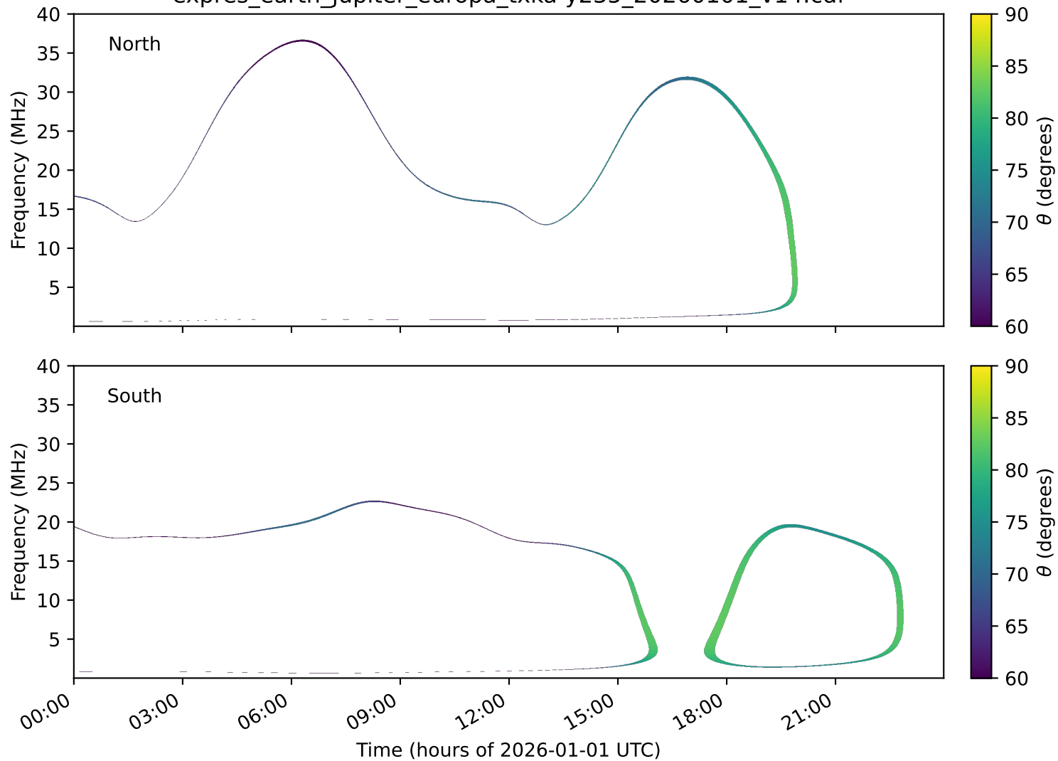
expres_earth_jupiter_europa_txka-y235_20260101_v14.cdf
